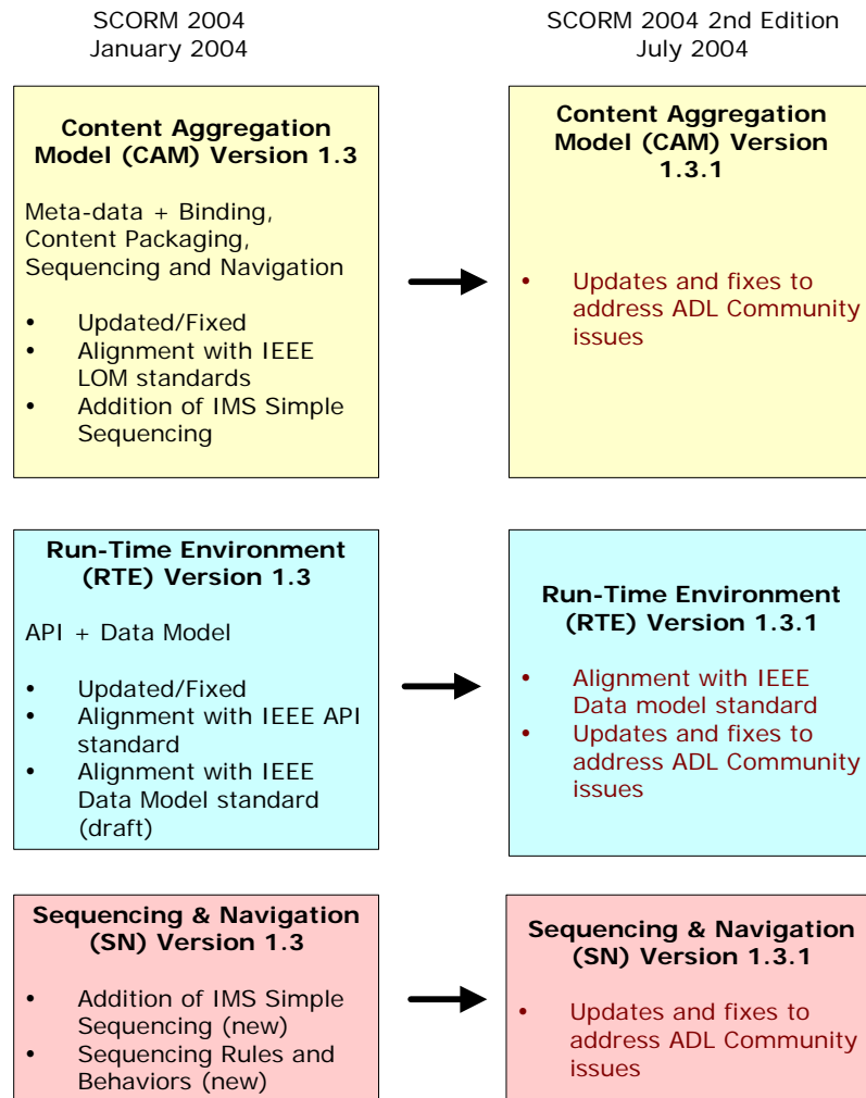
Figure 1.2a: SCORM Evolution
